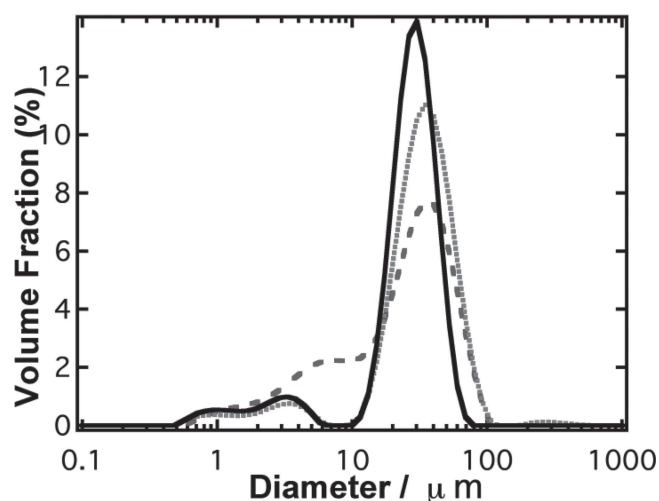
Figure 3. Volume averaged size distribution of the microcapsules in water. Oil-to-zein ratios: 1.75: solid, 4.5: dashed, 7.8: dotted. The O/Z 1.75 curve corresponds to an initial 3% zein mixture, while the other two to a 2%. For identical preparation conditions, the particle size distribution is similar.
